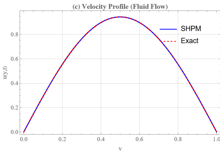
Figure (c) presents the velocity profile showing perfect agreement between SHPM and exact solutions.
